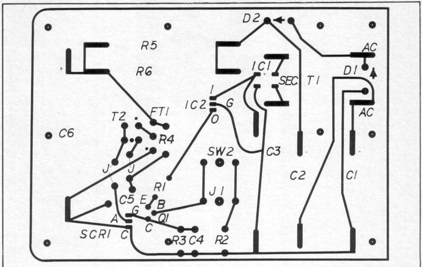
This is the PC pattern and parts placement diagram, shown actual size. Use this pattern to make your PC board. Refer to CINEMAGIC #13, page 29 if you're not familiar with the procedure for etching a PC board. Drill only the dots with the white dots in the center. Make absolutely sure that all parts are properly in place before plugging this unit in. Make especially sure that C-1, C-2 and C-6 are correctly installed because these parts could explode if improperly installed.
